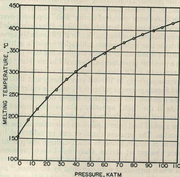
FIG. 6. Fusion curve of indium.
